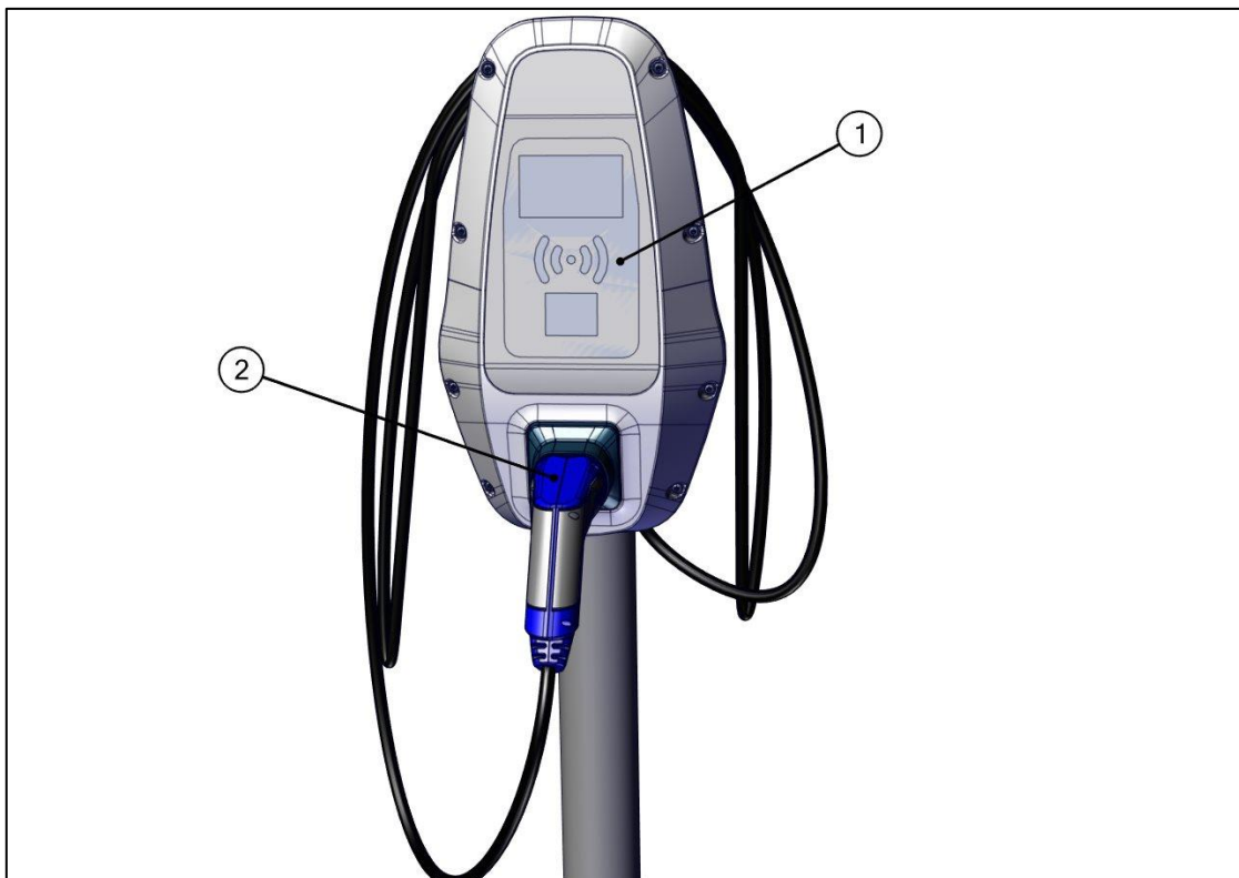
Figure 20 Charging cable
